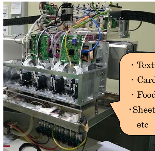
1800mm textile Color-printing device top
